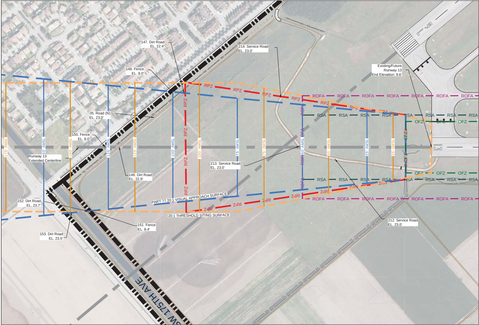
Plan View - R/W 13 Scale: 1"=200'
