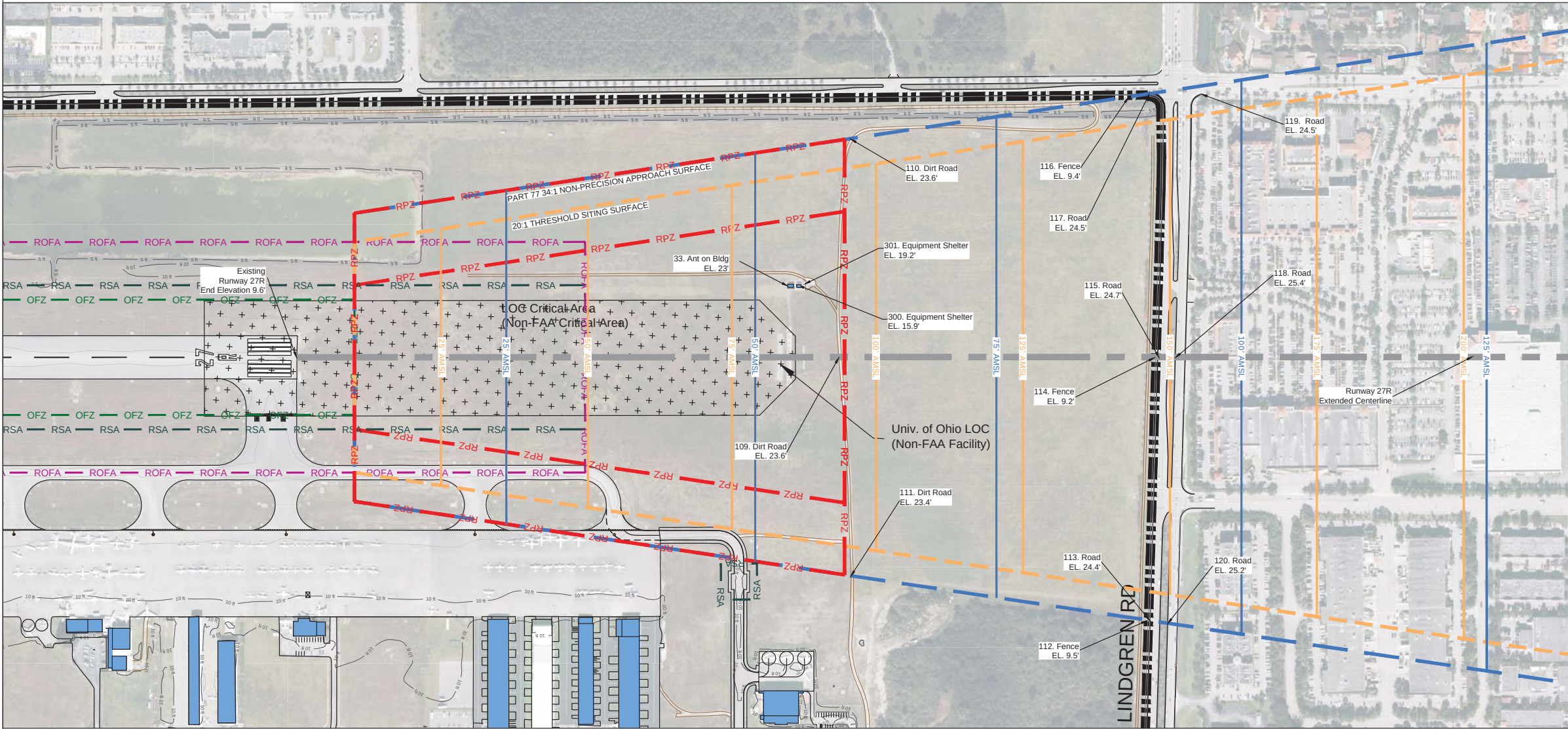
Plan View - R/W 27R Scale: 1"=200'
