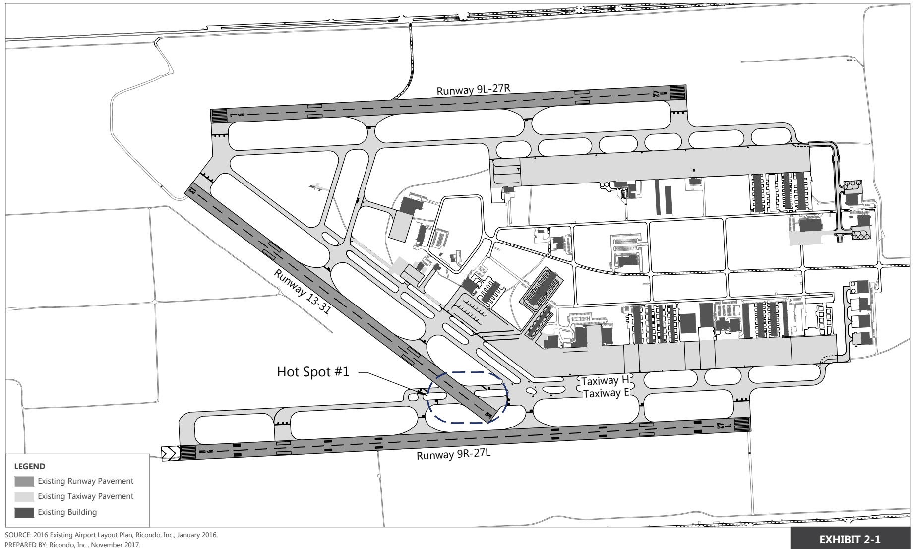
Existing Airfield Pavement Geometry
