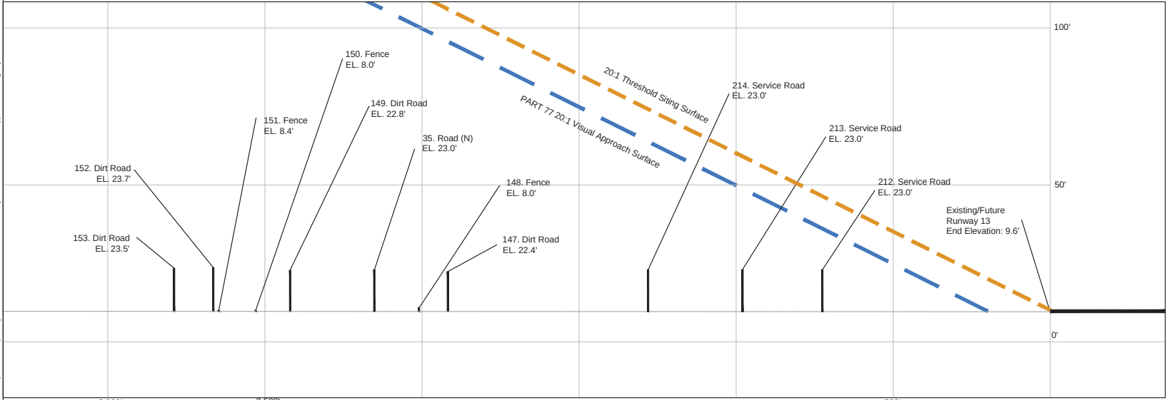
Profile View - R/W 13 Scale: 1"=200' (H); 1"=20' (V)
